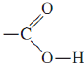
carboxyl group
