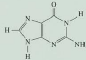
Guanine
