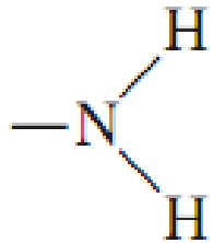
amino group
